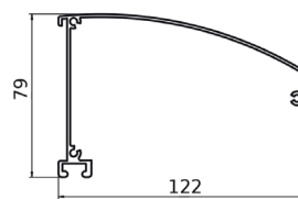
SEMI-ROUND CASSETTE
