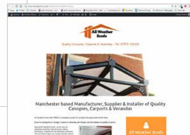
Example webpages
