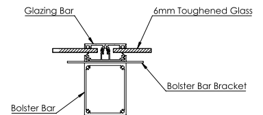
Bolster Bar, Glazing Bar & Glass Sheet Connection
