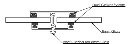
Roof Glazing Bar & Sheet Section
