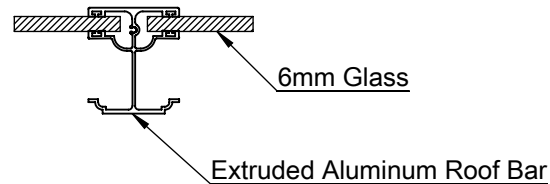
Roof Bar & Sheet Section
