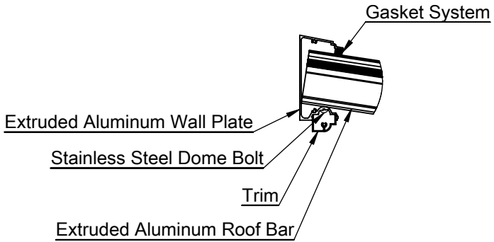
Wall Plate & Roof Bar Section
