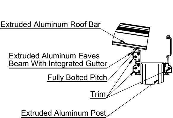
Eaves Beam Roof Bar & Post Section
