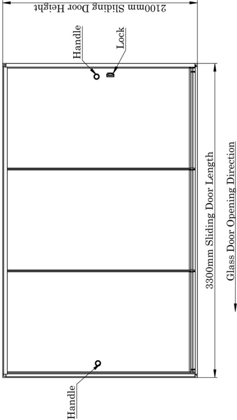
Front Sliding Door
